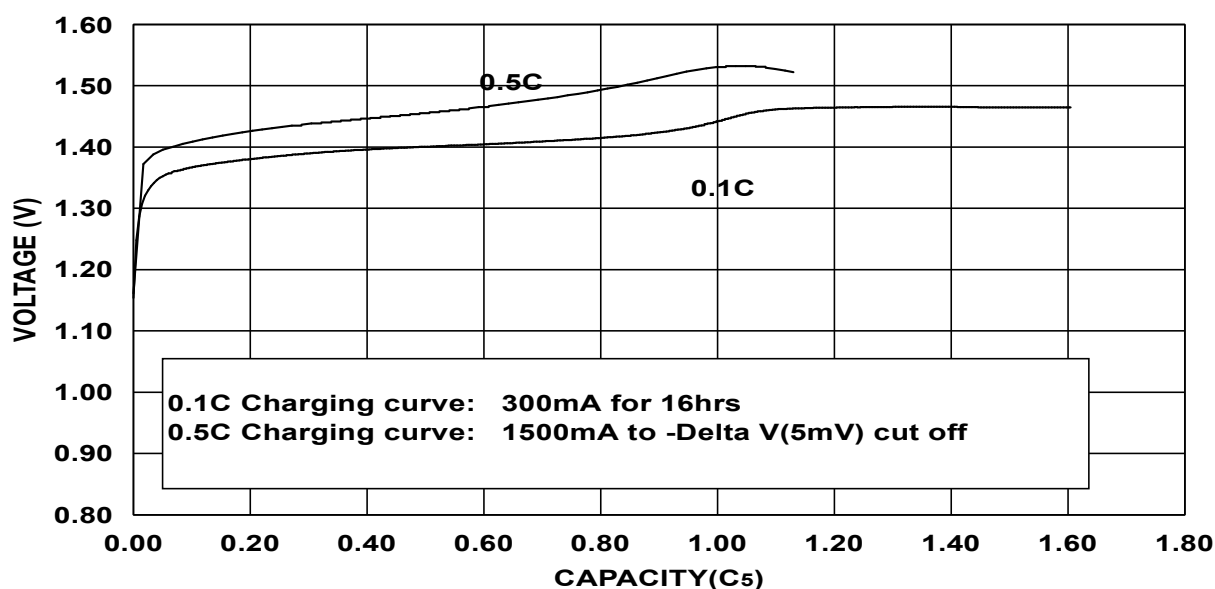
CHARGING CURVE OF BPI-43SC3000XPmAh CELL
