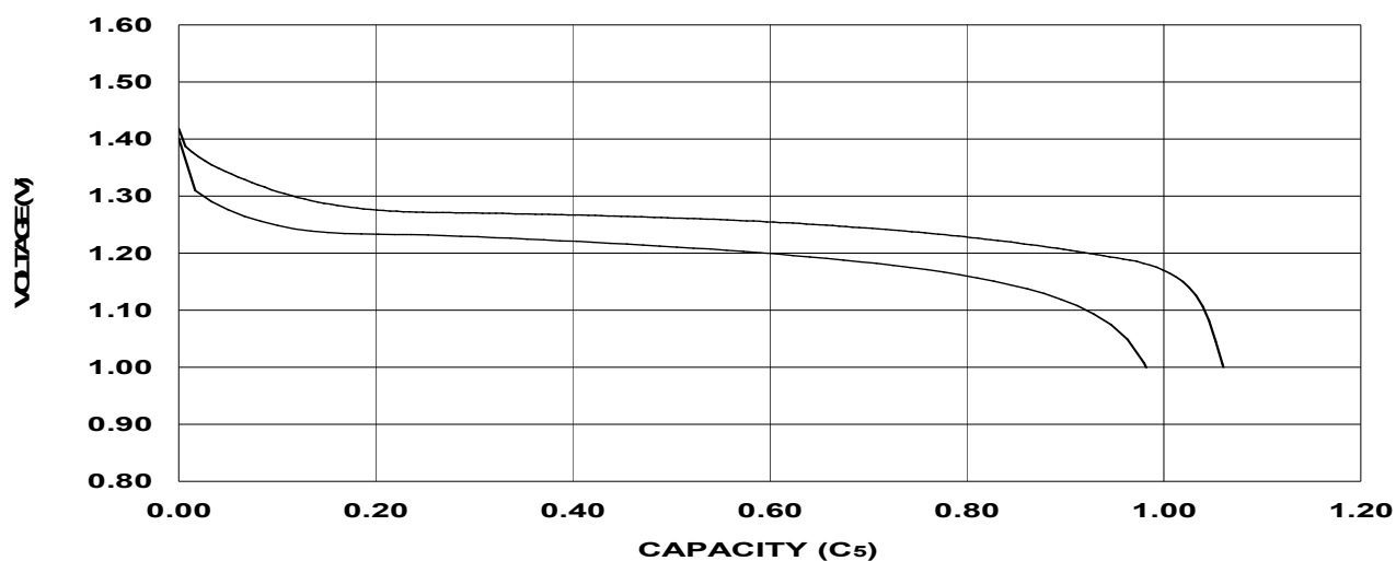
DISCHARGE CHARACTERISTICS OF BPI-43SC3000XP mAh CELL
