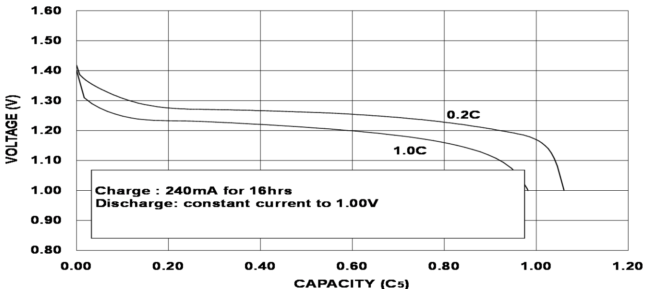
DISCHARGE CHARACTERISTICS OF BPI-49AA2400 mAh CELL
