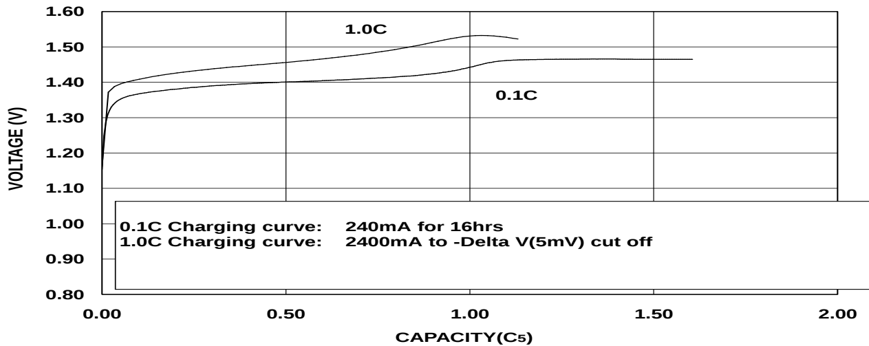
CHARGING CURVE OF BPI-49AA2400 mAh CELL
